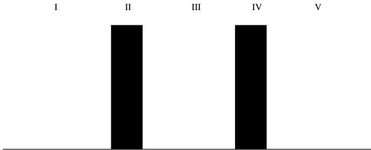
Fig. 2. The potential of Eq. (3.4).
