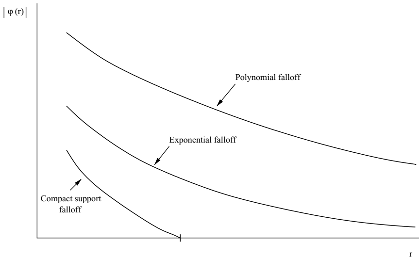
Fig. 1. Schematic representation of the three regimes of particle localization.
